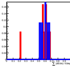
Deposit Energy[2511.89GeV, 3981.07GeV] in L9
