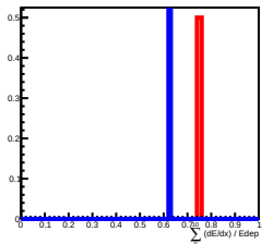
Deposit Energy[3981.07GeV, 6309.57GeV] in L10
