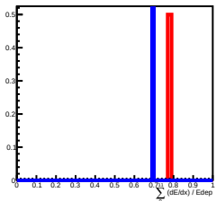
Deposit Energy[3981.07GeV, 6309.57GeV] in L11
