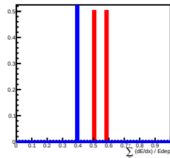
Deposit Energy[3981.07GeV, 6309.57GeV] in L12
