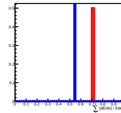
Deposit Energy[3981.07GeV, 6309.57GeV] in L9
