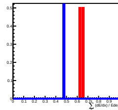
Deposit Energy[3981.07GeV, 6309.57GeV] in L13
