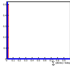
Deposit Energy[3981.07GeV, 6309.57GeV] in L7
