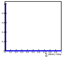
Deposit Energy[3981.07GeV, 6309.57GeV] in L5
