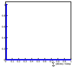
Deposit Energy[3981.07GeV, 6309.57GeV] in L6
