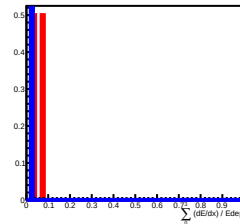
Deposit Energy[3981.07GeV, 6309.57GeV] in L8
