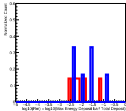
Deposit Energy[25.12GeV, 39.81GeV] in L10
