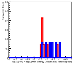
Deposit Energy[25.12GeV, 39.81GeV] in L11
