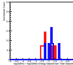
Deposit Energy[25.12GeV, 39.81GeV] in L12
