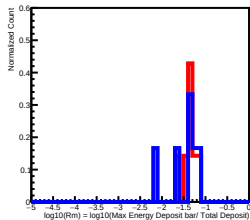
Deposit Energy[25.12GeV, 39.81GeV] in L5
