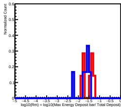
Deposit Energy[25.12GeV, 39.81GeV] in L6
