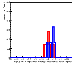
Deposit Energy[25.12GeV, 39.81GeV] in L8
