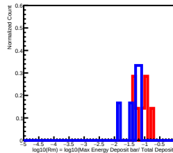
Deposit Energy[25.12GeV, 39.81GeV] in L7
