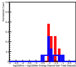
Deposit Energy[63.10GeV, 100.00GeV] in L11
