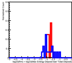
Deposit Energy[63.10GeV, 100.00GeV] in L10
