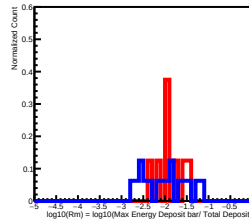
Deposit Energy[63.10GeV, 100.00GeV] in L13
