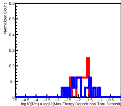
Deposit Energy[63.10GeV, 100.00GeV] in L12
