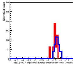
Deposit Energy[158.49GeV, 251.19GeV] in L7
