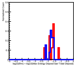
Deposit Energy[158.49GeV, 251.19GeV] in L11
