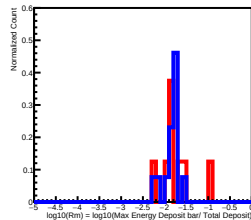
Deposit Energy[158.49GeV, 251.19GeV] in L12
