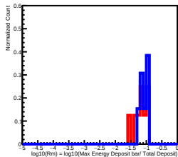
Deposit Energy[158.49GeV, 251.19GeV] in L5
