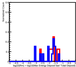
Deposit Energy[158.49GeV, 251.19GeV] in L1
