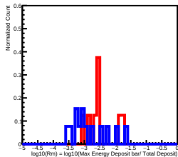
Deposit Energy[158.49GeV, 251.19GeV] in L0
