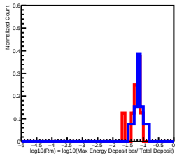
Deposit Energy[158.49GeV, 251.19GeV] in L6
