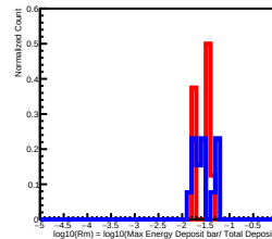
Deposit Energy[158.49GeV, 251.19GeV] in L9
