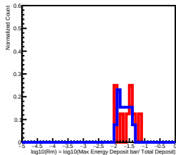
Deposit Energy[158.49GeV, 251.19GeV] in L10
