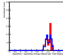
Deposit Energy[251.19GeV, 398.11GeV] in L9
