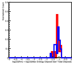
Deposit Energy[251.19GeV, 398.11GeV] in L6
