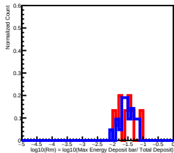
Deposit Energy[251.19GeV, 398.11GeV] in L10
