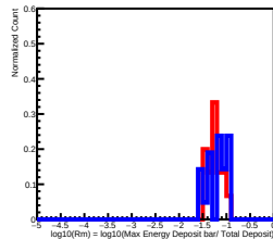
Deposit Energy[251.19GeV, 398.11GeV] in L7
