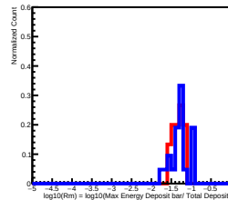
Deposit Energy[251.19GeV, 398.11GeV] in L8
