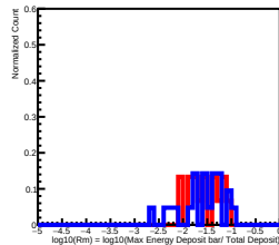
Deposit Energy[251.19GeV, 398.11GeV] in L2
