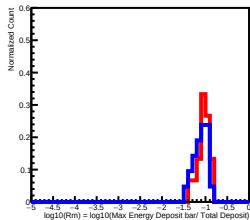
Deposit Energy[251.19GeV, 398.11GeV] in L5
