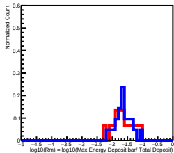
Deposit Energy[251.19GeV, 398.11GeV] in L11
