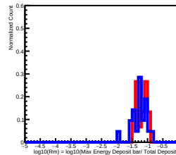
Deposit Energy[251.19GeV, 398.11GeV] in L3
