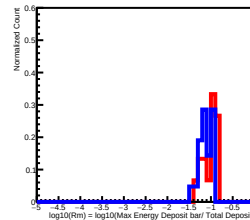
Deposit Energy[251.19GeV, 398.11GeV] in L4
