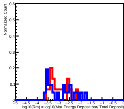
Deposit Energy[251.19GeV, 398.11GeV] in L0
