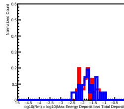
Deposit Energy[251.19GeV, 398.11GeV] in L13
