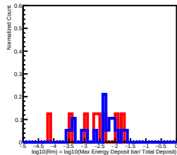
Deposit Energy[1584.89GeV, 2511.89GeV] in L1
