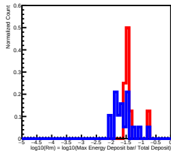
Deposit Energy[1584.89GeV, 2511.89GeV] in L12
