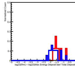
Deposit Energy[1584.89GeV, 2511.89GeV] in L13
