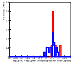
Deposit Energy[1584.89GeV, 2511.89GeV] in L11
