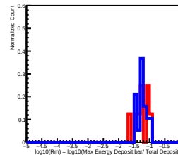
Deposit Energy[1584.89GeV, 2511.89GeV] in L8
