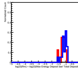
Deposit Energy[1584.89GeV, 2511.89GeV] in L4
