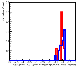
Deposit Energy[1584.89GeV, 2511.89GeV] in L5
