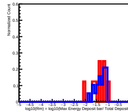
Deposit Energy[1584.89GeV, 2511.89GeV] in L3
