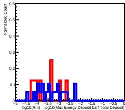
Deposit Energy[1584.89GeV, 2511.89GeV] in L0
