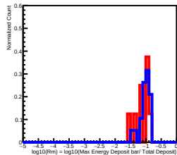
Deposit Energy[1584.89GeV, 2511.89GeV] in L6
