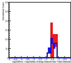
Deposit Energy[1584.89GeV, 2511.89GeV] in L10
