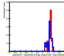
Deposit Energy[1584.89GeV, 2511.89GeV] in L9
