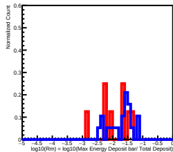
Deposit Energy[1584.89GeV, 2511.89GeV] in L2
