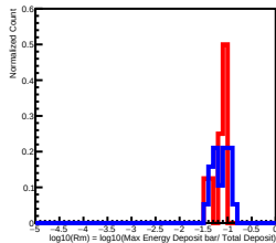
Deposit Energy[1584.89GeV, 2511.89GeV] in L7
