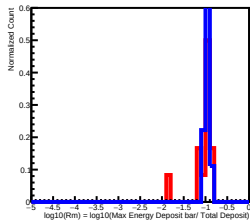
Deposit Energy[2511.89GeV, 3981.07GeV] in L5
