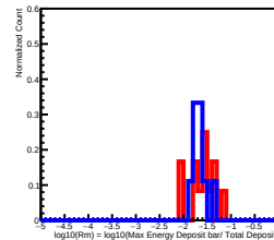
Deposit Energy[2511.89GeV, 3981.07GeV] in L13
