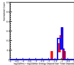
Deposit Energy[2511.89GeV, 3981.07GeV] in L7
