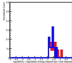
Deposit Energy[2511.89GeV, 3981.07GeV] in L12
