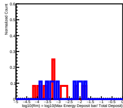
Deposit Energy[2511.89GeV, 3981.07GeV] in L1
