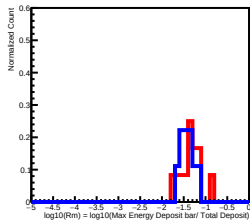
Deposit Energy[2511.89GeV, 3981.07GeV] in L10
