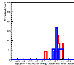
Deposit Energy[2511.89GeV, 3981.07GeV] in L3
