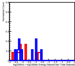
Deposit Energy[2511.89GeV, 3981.07GeV] in L0
