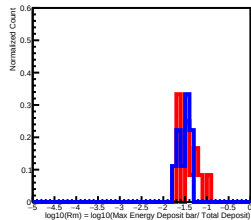
Deposit Energy[2511.89GeV, 3981.07GeV] in L11
