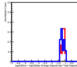
Deposit Energy[2511.89GeV, 3981.07GeV] in L8
