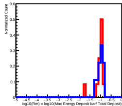
Deposit Energy[2511.89GeV, 3981.07GeV] in L6
