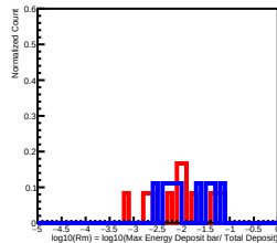
Deposit Energy[2511.89GeV, 3981.07GeV] in L2
