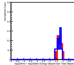
Deposit Energy[2511.89GeV, 3981.07GeV] in L9
