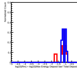
Deposit Energy[2511.89GeV, 3981.07GeV] in L4
