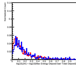
Deposit Energy[15.85GeV, 25.12GeV] in L13
