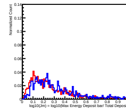
Deposit Energy[15.85GeV, 25.12GeV] in L9
