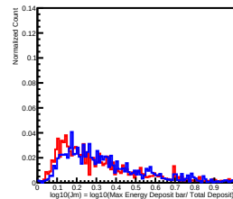
Deposit Energy[15.85GeV, 25.12GeV] in L8
