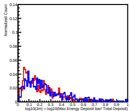
Deposit Energy[15.85GeV, 25.12GeV] in L11
