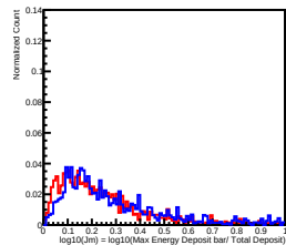
Deposit Energy[15.85GeV, 25.12GeV] in L10
