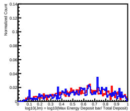
Deposit Energy[15.85GeV, 25.12GeV] in L6
