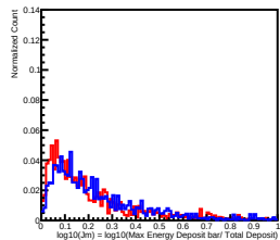
Deposit Energy[15.85GeV, 25.12GeV] in L12
