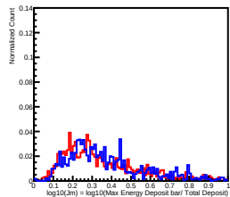
Deposit Energy[15.85GeV, 25.12GeV] in L7
