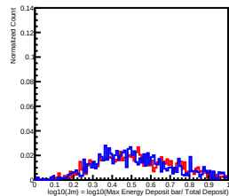
Deposit Energy[15.85GeV, 25.12GeV] in L5
