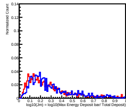
Deposit Energy[25.12GeV, 39.81GeV] in L10
