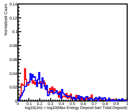
Deposit Energy[25.12GeV, 39.81GeV] in L11
