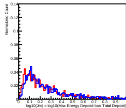
Deposit Energy[25.12GeV, 39.81GeV] in L12
