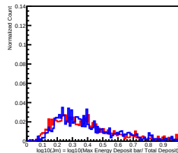
Deposit Energy[39.81GeV, 63.10GeV] in L8
