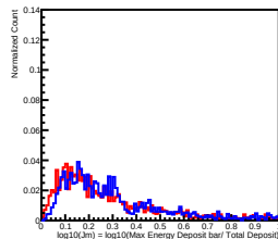
Deposit Energy[39.81GeV, 63.10GeV] in L12
