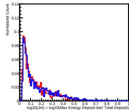
Deposit Energy[39.81GeV, 63.10GeV] in L5
