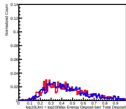
Deposit Energy[39.81GeV, 63.10GeV] in L7
