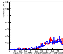
Deposit Energy[39.81GeV, 63.10GeV] in L9
