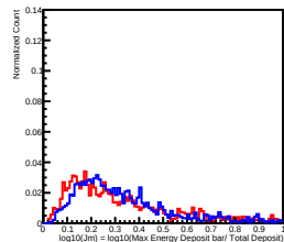
Deposit Energy[39.81GeV, 63.10GeV] in L10
