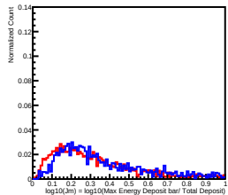
Deposit Energy[158.49GeV, 251.19GeV] in L12
