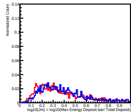
Deposit Energy[158.49GeV, 251.19GeV] in L10
