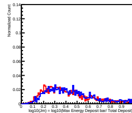
Deposit Energy[158.49GeV, 251.19GeV] in L9
