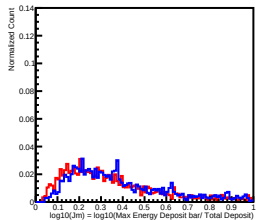
Deposit Energy[158.49GeV, 251.19GeV] in L11
