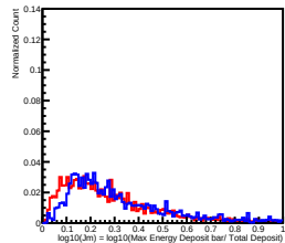
Deposit Energy[158.49GeV, 251.19GeV] in L13
