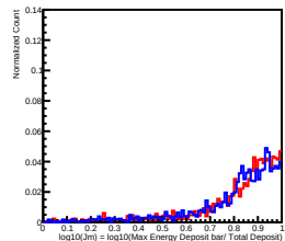
Deposit Energy[398.11GeV, 630.96GeV] in L5
