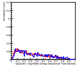
Deposit Energy[398.11GeV, 630.96GeV] in L2
