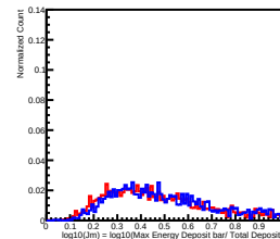
Deposit Energy[398.11GeV, 630.96GeV] in L9
