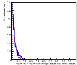
Deposit Energy[398.11GeV, 630.96GeV] in L0
