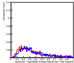
Deposit Energy[398.11GeV, 630.96GeV] in L12
