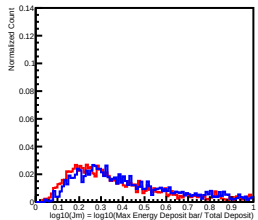
Deposit Energy[398.11GeV, 630.96GeV] in L11
