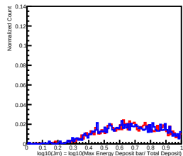
Deposit Energy[398.11GeV, 630.96GeV] in L7
