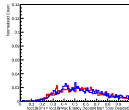
Deposit Energy[398.11GeV, 630.96GeV] in L8
