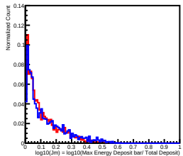
Deposit Energy[398.11GeV, 630.96GeV] in L1
