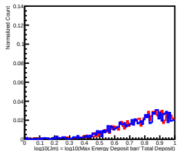
Deposit Energy[398.11GeV, 630.96GeV] in L6
