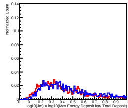
Deposit Energy[398.11GeV, 630.96GeV] in L10
