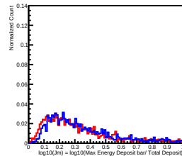
Deposit Energy[398.11GeV, 630.96GeV] in L13
