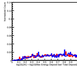
Deposit Energy[398.11GeV, 630.96GeV] in L3
