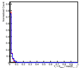
Deposit Energy[1000.00GeV, 1584.89GeV] in L5
