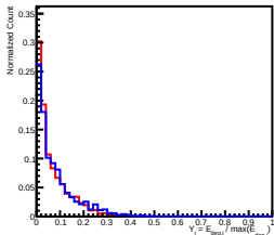
Deposit Energy[1000.00GeV, 1584.89GeV] in L6
