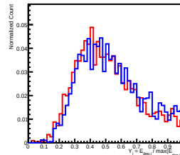
Deposit Energy[1000.00GeV, 1584.89GeV] in L9
