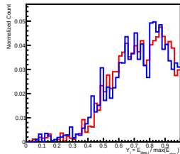
Deposit Energy[1000.00GeV, 1584.89GeV] in L7
