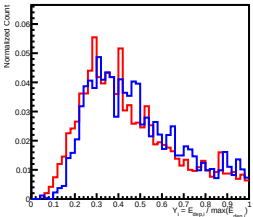
Deposit Energy[1000.00GeV, 1584.89GeV] in L10
