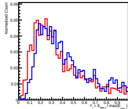
Deposit Energy[1000.00GeV, 1584.89GeV] in L12
