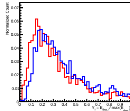
Deposit Energy[1000.00GeV, 1584.89GeV] in L13
