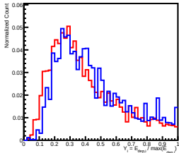
Deposit Energy[1000.00GeV, 1584.89GeV] in L11
