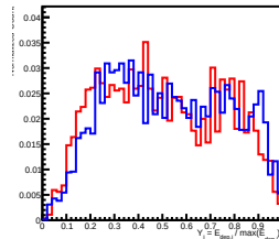
Deposit Energy[1000.00GeV, 1584.89GeV] in L8
