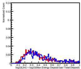
Deposit Energy[2511.89GeV, 3981.07GeV] in L11
