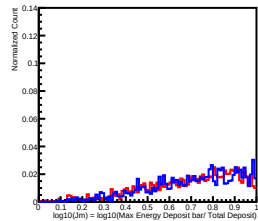
Deposit Energy[2511.89GeV, 3981.07GeV] in L9
