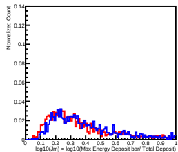
Deposit Energy[2511.89GeV, 3981.07GeV] in L12
