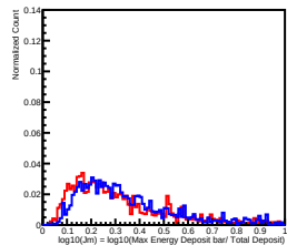
Deposit Energy[2511.89GeV, 3981.07GeV] in L13
