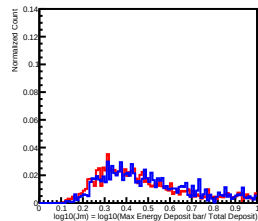
Deposit Energy[2511.89GeV, 3981.07GeV] in L10
