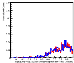
Deposit Energy[2511.89GeV, 3981.07GeV] in L7
