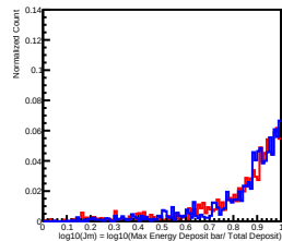
Deposit Energy[2511.89GeV, 3981.07GeV] in L5
