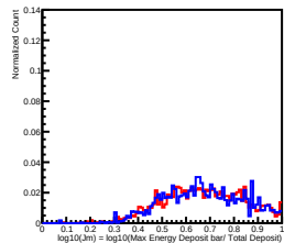
Deposit Energy[2511.89GeV, 3981.07GeV] in L8
