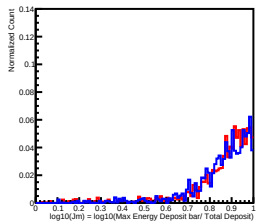
Deposit Energy[2511.89GeV, 3981.07GeV] in L6
