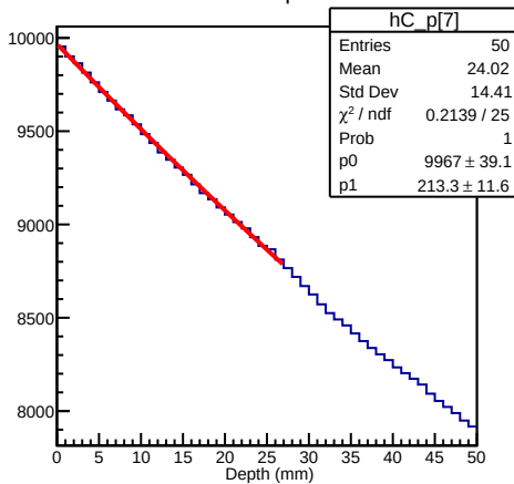
80 GeV Proton Depth Distribution
