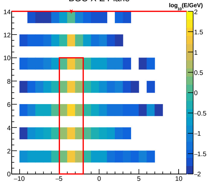
BGO X-Z Plane
