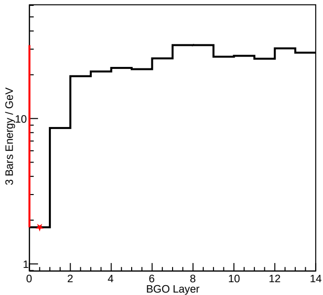
BGO Core Axis Energy Deposit
