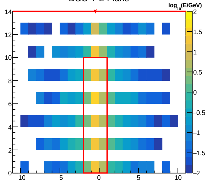
BGO Y-Z Plane
