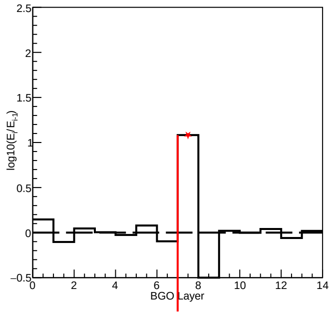
BGO Core Axis Energy Deposit Change Rate
