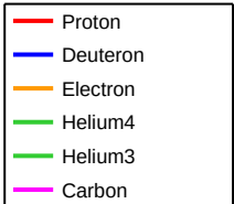
IncidentParticle 20GeV
