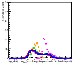
400 GeV incident in L0
