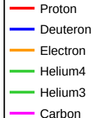
IncidentParticle 70GeV
