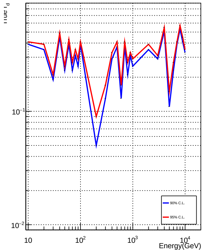
Sensitivity Curve from N_{\text{int}}
