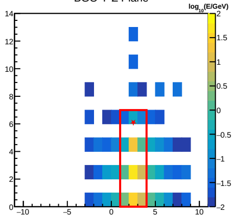
BGO Y-Z Plane
