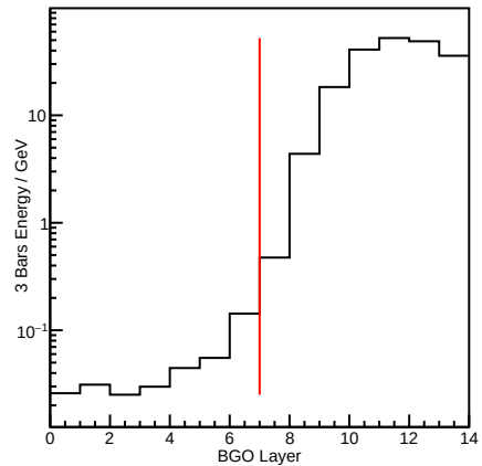
BGO Core Axis Energy Deposit
