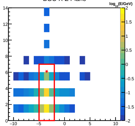
BGO X-Z Plane
