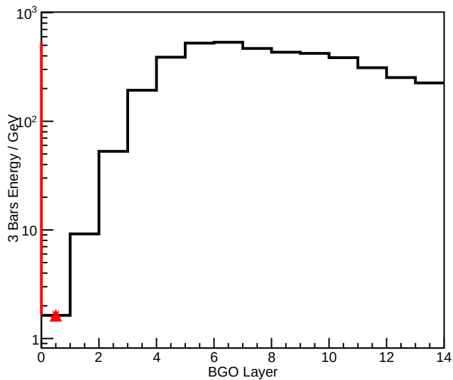
BGO Core Axis Energy Deposit
