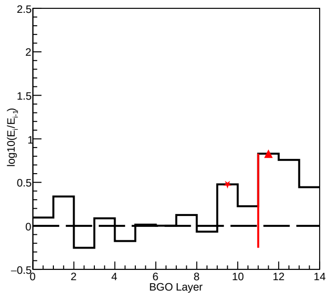
BGO Core Axis Energy Deposit Change Rate
