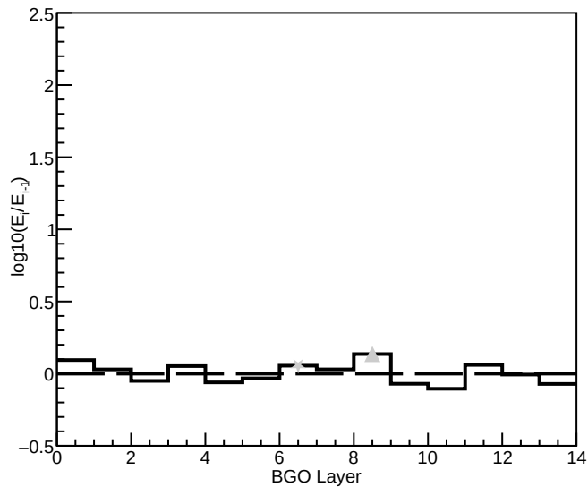
BGO Core Axis Energy Deposit Change Rate
