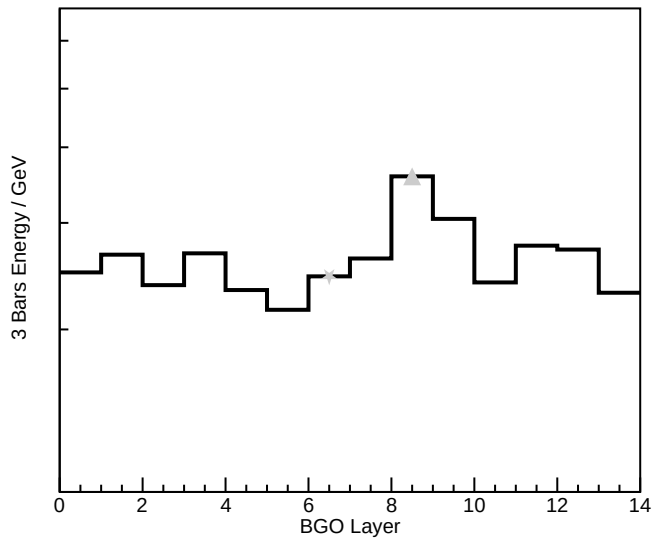
BGO Core Axis Energy Deposit
