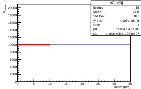
10 GeV Carbon Depth Distribution
