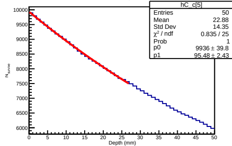
60 GeV Carbon Depth Distribution
