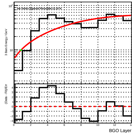
BGO Core Axis Energy Deposit
