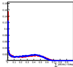
Deposit Energy[1000.00GeV, 1584.89GeV] in L12
