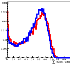
Deposit Energy[1000.00GeV, 1584.89GeV] in L9
