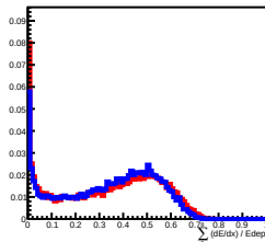
Deposit Energy[1000.00GeV, 1584.89GeV] in L13
