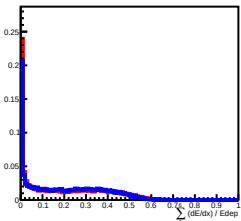
Deposit Energy[1000.00GeV, 1584.89GeV] in L11
