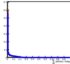
Deposit Energy[1000.00GeV, 1584.89GeV] in L8
