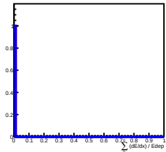
Deposit Energy[1000.00GeV, 1584.89GeV] in L5
