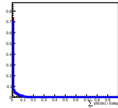
Deposit Energy[1000.00GeV, 1584.89GeV] in L7
