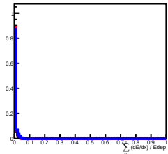
Deposit Energy[1000.00GeV, 1584.89GeV] in L6
