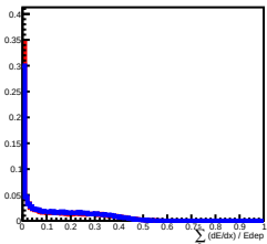
Deposit Energy[1000.00GeV, 1584.89GeV] in L10
