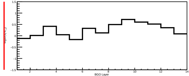
BGO Core Axis Energy Deposit Change Rate
