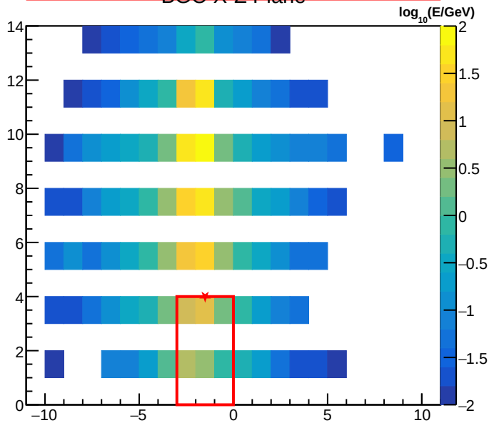
BGO X-Z Plane
