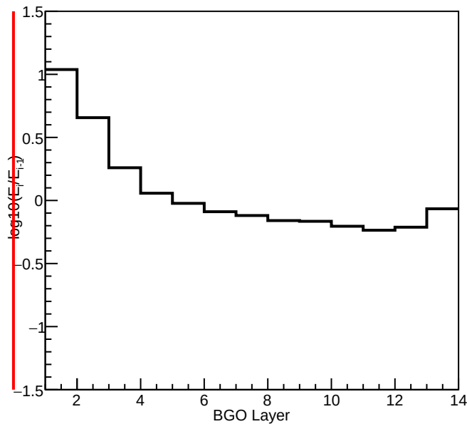
BGO Core Axis Energy Deposit Change Rate
