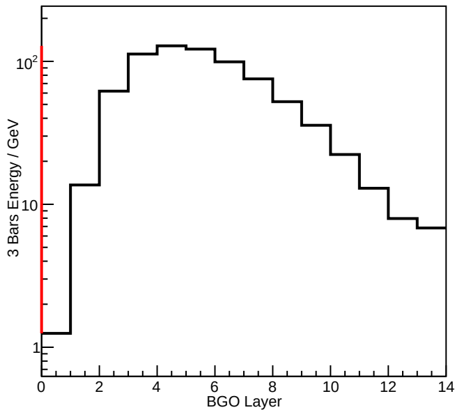
BGO Core Axis Energy Deposit
