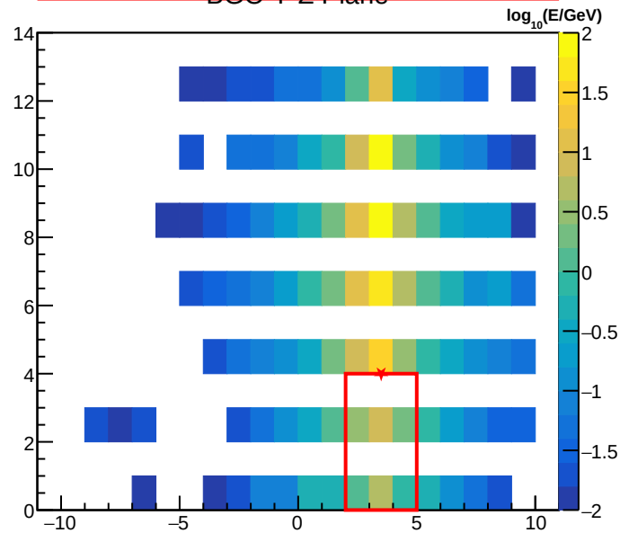
BGO Y-Z Plane
