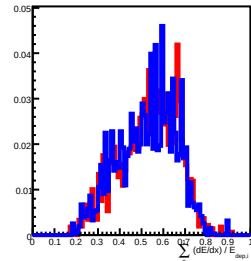
Deposit Energy[630.96GeV, 1000.00GeV] in L6
