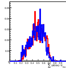
Deposit Energy[630.96GeV, 1000.00GeV] in L8
