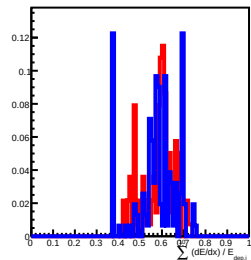
Deposit Energy[630.96GeV, 1000.00GeV] in L10
