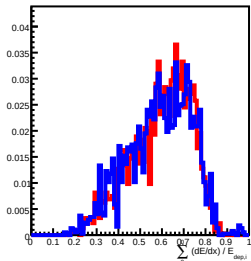
Deposit Energy[630.96GeV, 1000.00GeV] in L5
