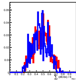
Deposit Energy[630.96GeV, 1000.00GeV] in L7
