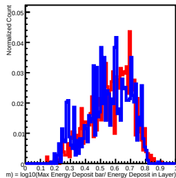
Deposit Energy[630.96GeV, 1000.00GeV] in L9
