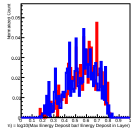
Deposit Energy[630.96GeV, 1000.00GeV] in L10
