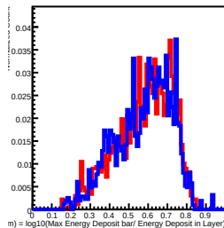
Deposit Energy[630.96GeV, 1000.00GeV] in L6
