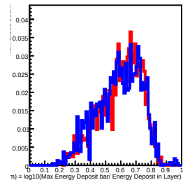
Deposit Energy[630.96GeV, 1000.00GeV] in L5
