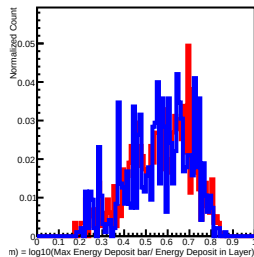
Deposit Energy[630.96GeV, 1000.00GeV] in L7
