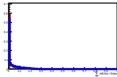
Deposit Energy[1000.00GeV, 1584.89GeV] in L8
