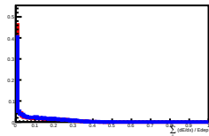
Deposit Energy[1000.00GeV, 1584.89GeV] in L9
