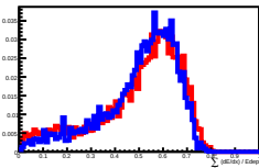
Deposit Energy[1000.00GeV, 1584.89GeV] in L10
