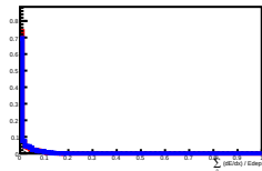
Deposit Energy[1000.00GeV, 1584.89GeV] in L7
