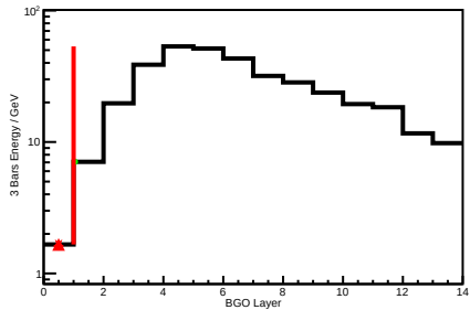
BGO Core Axis Energy Deposit
