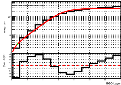
Accumulated Energy Deposit
