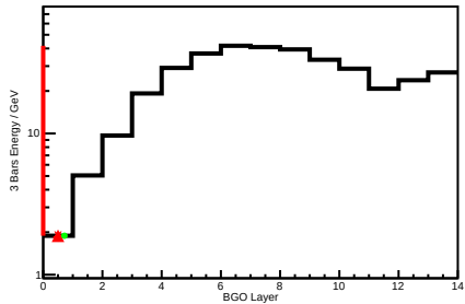
BGO Core Axis Energy Deposit
