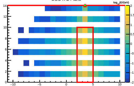
BGO X-Z Plane
