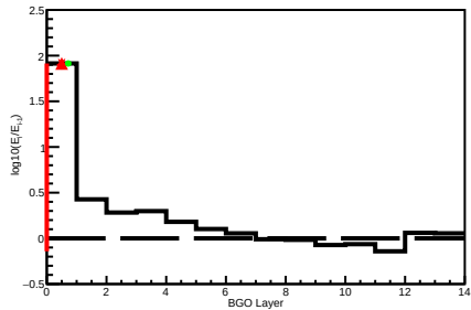
BGO Core Axis Energy Deposit Change Rate
