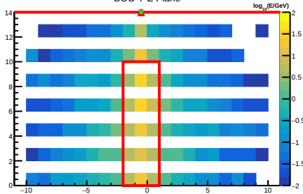
BGO Y-Z Plane
