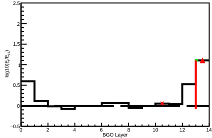
BGO Core Axis Energy Deposit Change Rate
