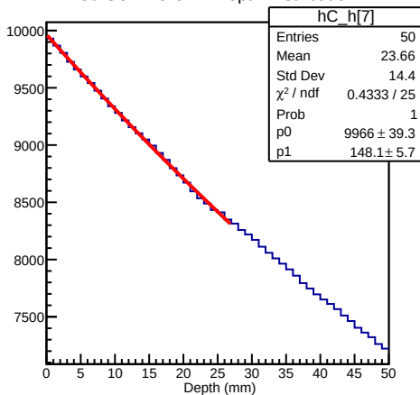
80 GeV Helium4 Depth Distribution
