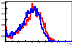
400 GeV incident in L12
