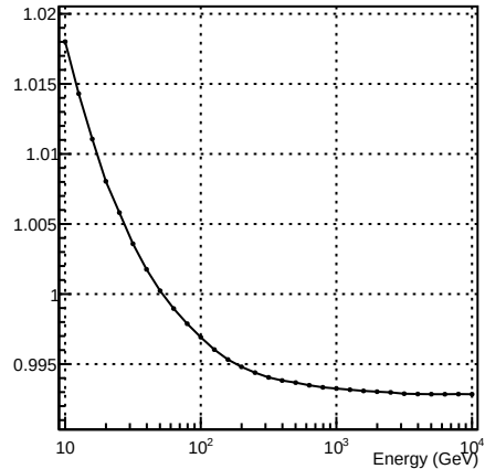
Correction Factor: QE Geant4.11/Meson Geant4.11
