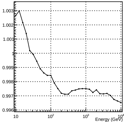
Correction Factor: PiKaon Geant4.11/Geant4.10
