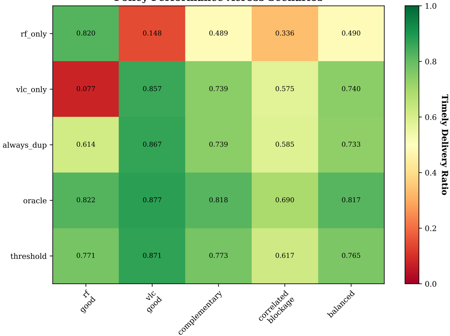
Policy Performance Across Scenarios
