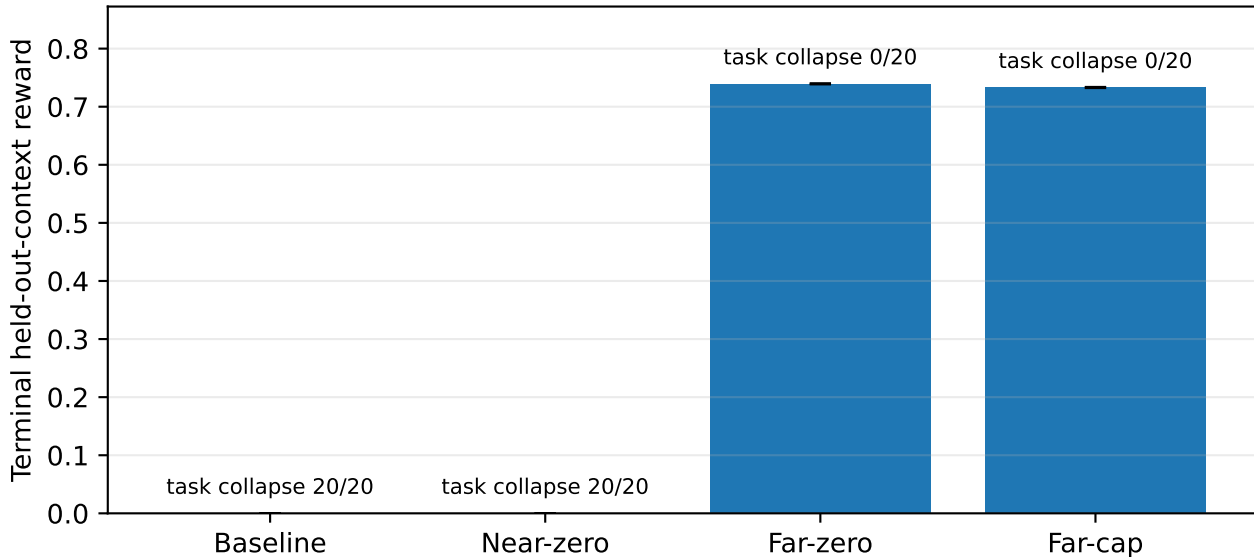
C-U1 E3 fixed-variance targeted intervention (20 paired seeds)
