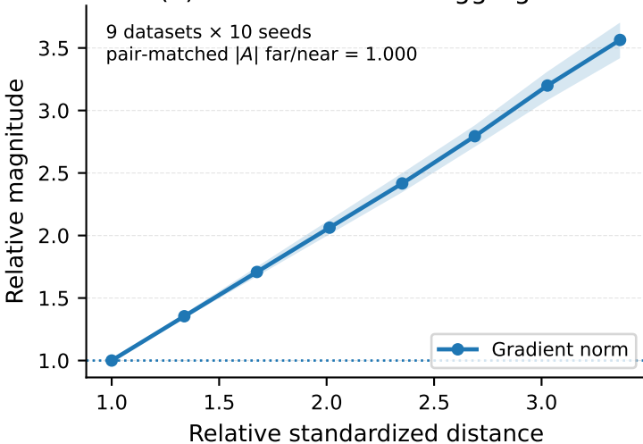
(a) D4RL locomotion aggregate
