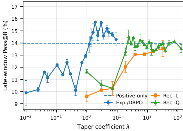
Figure 6: Countdown-0.5B taper-coefficient response. Late-window Pass@8 is shown against the taper coefficient \lambda under the fixed 1,200-step budget. Curves report two-seed late-window means; error bars span the paired seed values, and the dashed horizontal line denotes Positive-only. Exp./DRPO is shown over \lambda \in [0.01, 9.2103] , Reciprocal-Linear through 319, and Reciprocal-Quadratic through 1279.
