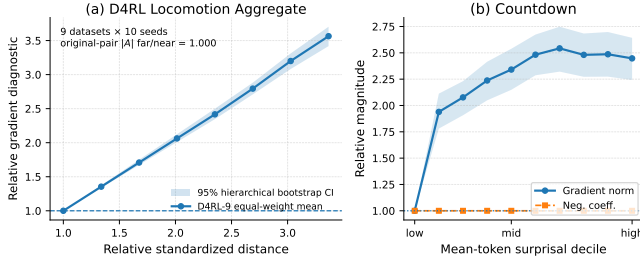
Figure 1: External diagnostic of far-field negative-update magnitude. (a) D4RL locomotion: equal-weight aggregate across HalfCheetah, Hopper, and Walker2d under the medium, medium-replay, and medium-expert datasets. For negative learned-critic advantages, each far transition is normalized by its original matched near partner within seed and dataset. The line reports the cross-dataset mean, the shaded region denotes a hierarchical bootstrap 95% confidence interval over datasets and seeds, and the matched far/near absolute-advantage ratio is reported as a diagnostic. (b) Countdown: relative implemented actor-gradient diagnostic and fixed negative coefficient magnitude as functions of current-policy mean-token surprisal deciles among verifier-matched unsuccessful responses. Values are normalized to the lowest-surprisal decile, and shaded regions denote puzzle-level bootstrap 95% confidence intervals.
