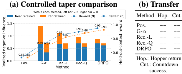
Figure 4. Controlled taper comparison and external transfer. (a) Matched operating-point comparison in the controlled taper protocol. For each method, the left bar is the near-field-retention matched operating point and the right bar is the aggregate-budget matched operating point. Bars decompose retained negative-update magnitude into near- and far-field components, and dashed traces report held-out-context reward. (b) Reserved external validation summary for Hopper and Countdown; dashes mark outcomes awaiting the corresponding formal runs.
