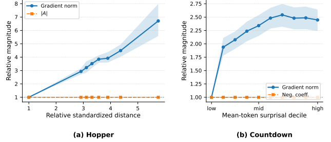
Figure 1. External diagnostic of far-field negative-update magnitude. (a) Hopper: relative implemented actor-gradient diagnostic and matched absolute advantage as functions of relative standardized distance for transitions with negative learned-critic advantages. Values are normalized to the near-field reference within each seed. Lines report averages across 10 seeds, and shaded regions denote seed-level bootstrap 95% confidence intervals. (b) Countdown: relative implemented actor-gradient diagnostic and fixed negative coefficient magnitude as functions of current-policy mean-token surprisal deciles among verifier-matched unsuccessful responses. Values are normalized to the lowest-surprisal decile, and shaded regions denote puzzle-level bootstrap 95% confidence intervals.
