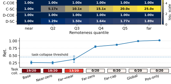
Figure 2. Controlled source isolation and causal transmission. Top: source-isolation factorization across learner-relative remoteness bins, normalized to the near bin. COE denotes coefficient magnitude and SC denotes policy-score response; C rows report the C-U1 continuous protocol, and D rows show the corresponding direct-softmax categorical reference. Bottom: C-U1 causal-intervention summary. Ret. denotes reward retention; points show 20-seed means with bootstrap confidence intervals, and Task coll. reports task-performance collapse counts.
