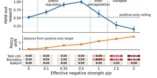
Figure 3: Stable extrapolation from controlled negative feedback. Increasing the effective negative strength q/p first improves held-out-context reward beyond the positive-only ceiling, then causes over-extrapolation and task-performance collapse. Policy shift measures displacement from the positive-only target. The color strip reports task collapse, boundary events, and NaN/Inf failures separately.
