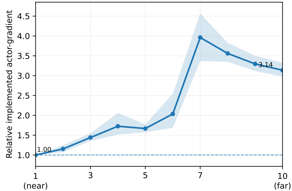
maze near->far = 3.14x
