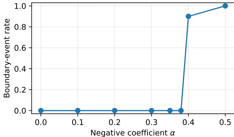
Support/variance boundary
